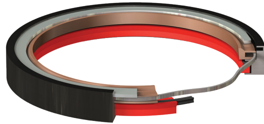
An A-Series, Style-2 Metallic Scraper. A serpentine spring is used on sizes ≥1.5" I.D.
