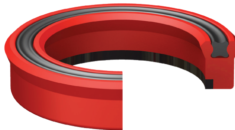
The standard compound for this seal is U2151, with an N6014 Expander and M1001 Anti-Extrusion Ring.
