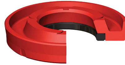
With M1001, Anti-Extrusion Ring (AER)
