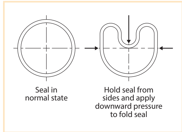
Figure SI-1 - Manual soft seal folding, for installation into a gland.
