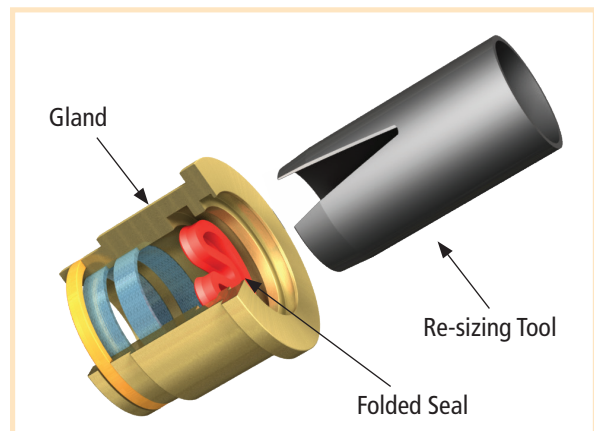
Figure SI-3 - Cut-away diagram showing an X-PAC® U-Cup, folded and positioned to fit into the groove.
