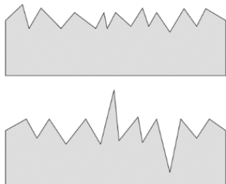
Fig 1. Example of two profiles that have the same R_a Note the large peak and valley on the second surface
