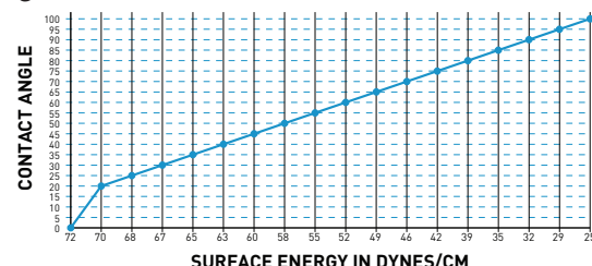
Figure 3 CONTACT ANGLE vs. SURFACE ENERGY
