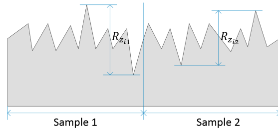
Fig 2. Visual representation of R_z
