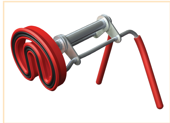
Figure SI-2 - An X-PAC® U-Cup, being folded using an installation tool.
